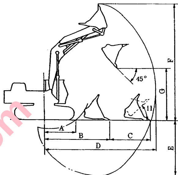
Tilt Dump Type
