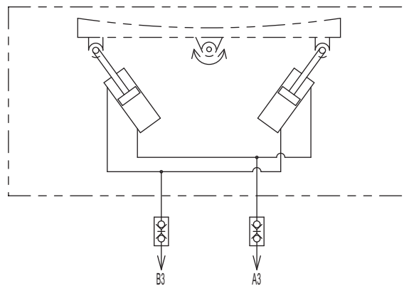
ANGLING PLOW
