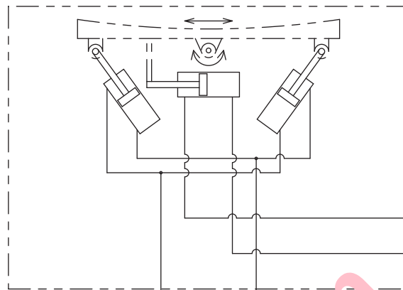
SIDE SLIDE ANGLING PLOW
