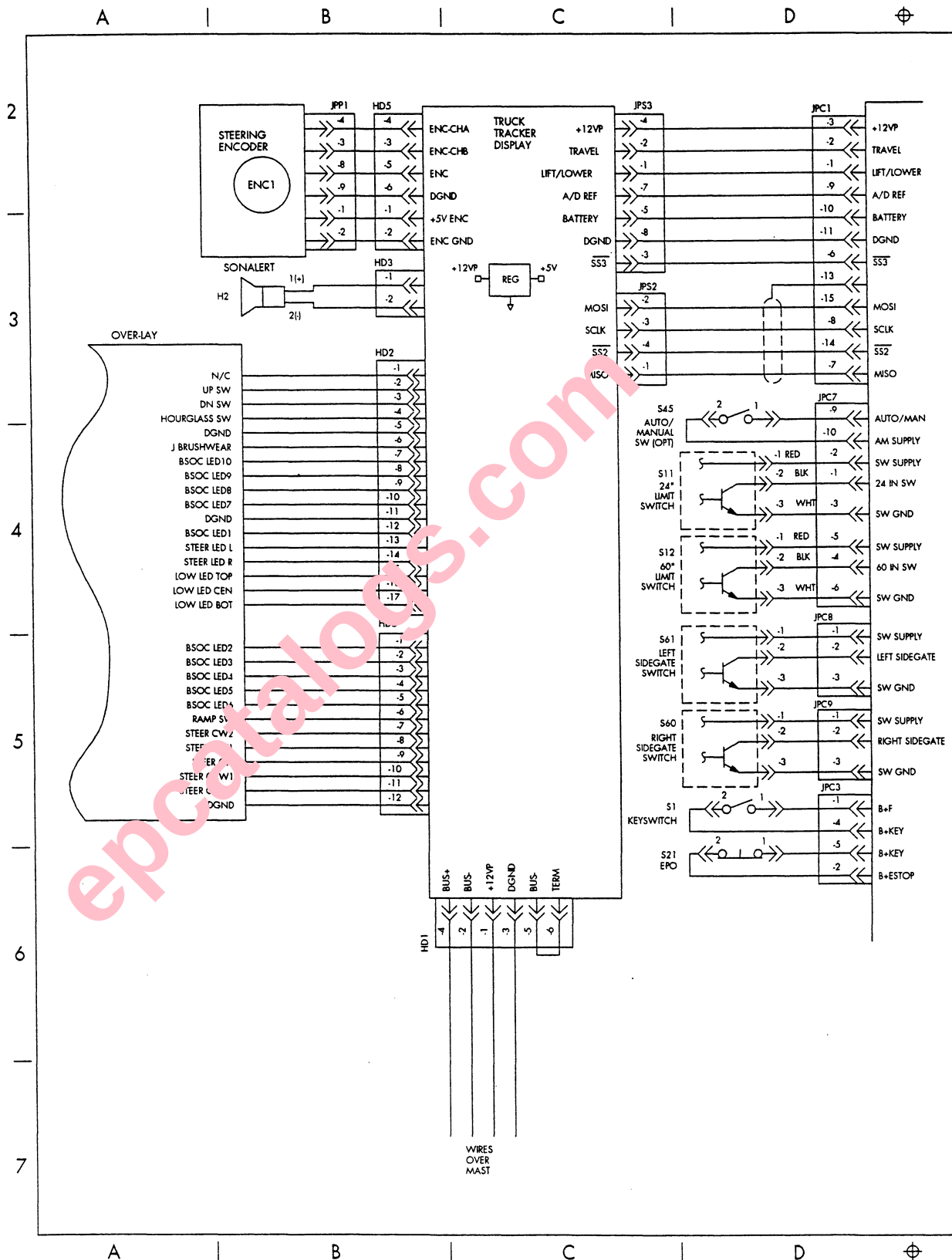
Figure 9-7: Electrical Schematic (sheet 1 of 3)
